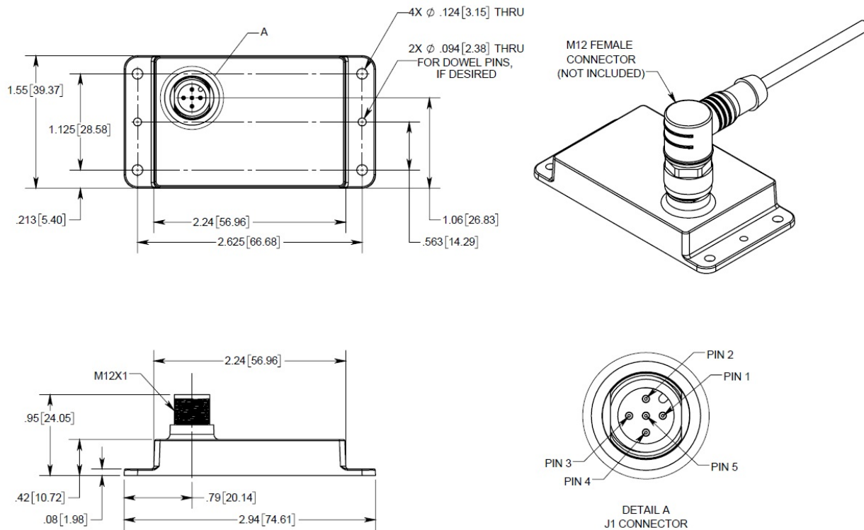
T7 Networked Absolute Inclinometer
