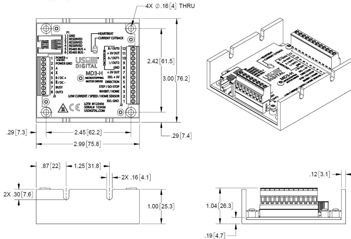
MD3 Microstepping Motor Driver
