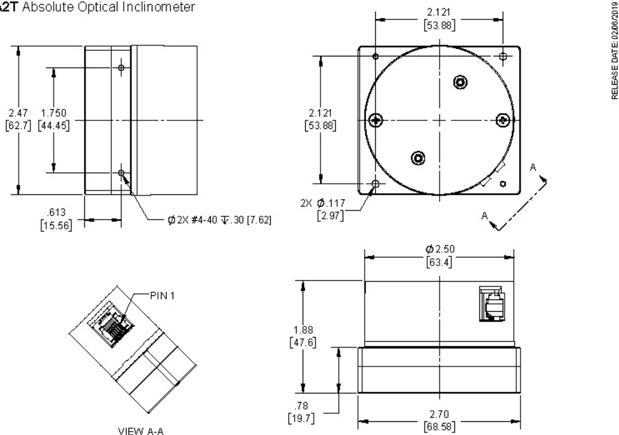
A2T Absolute Optical Inclinometer
